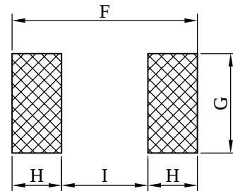
( PCB Pattern )
